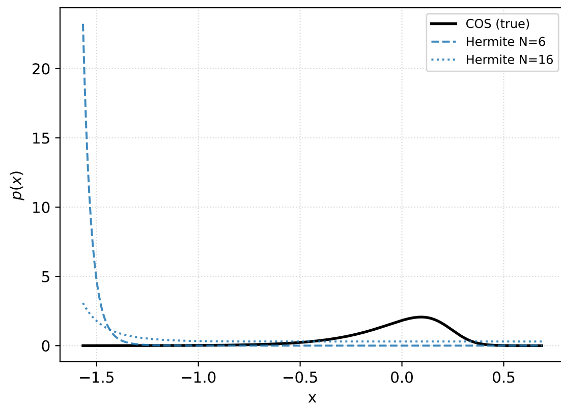
Figure 11: Density comparison — Heston (restricted)
