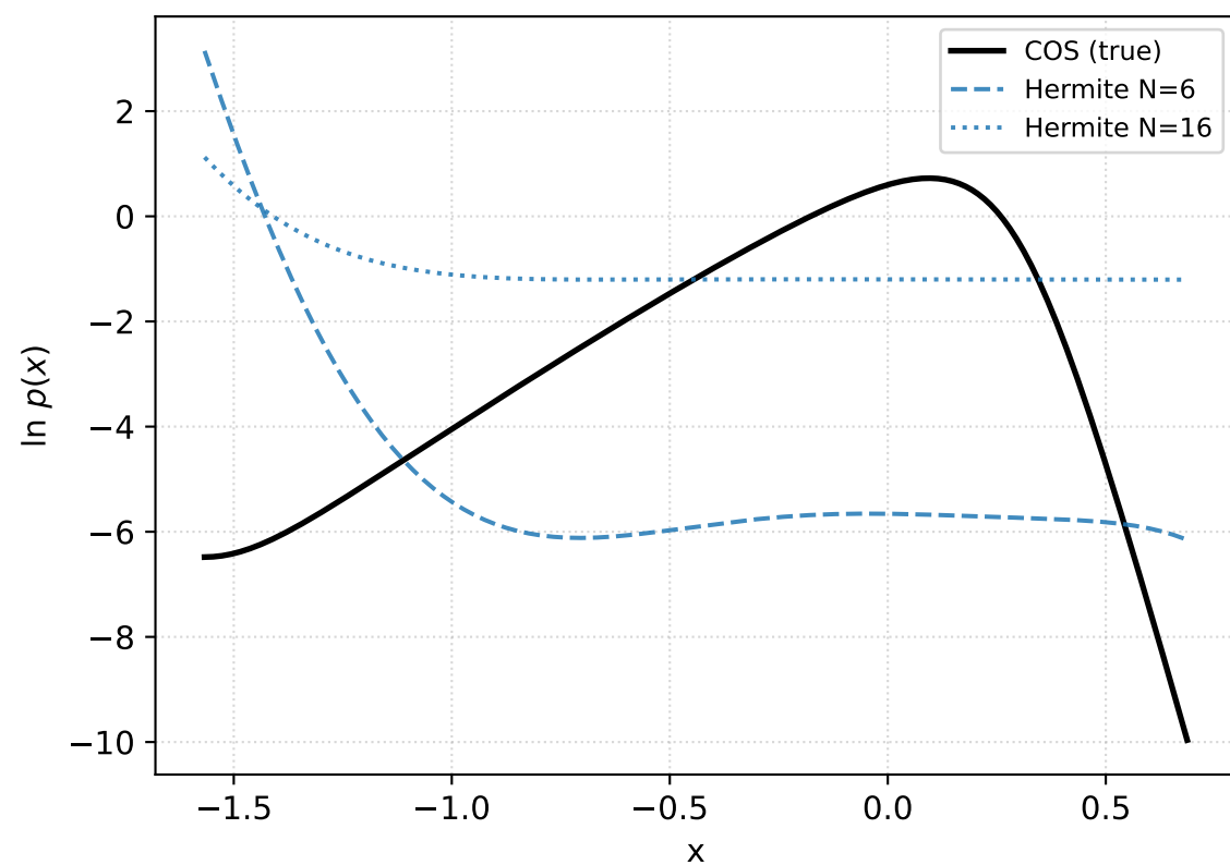
Figure 11: Density comparison — Heston (restricted)
